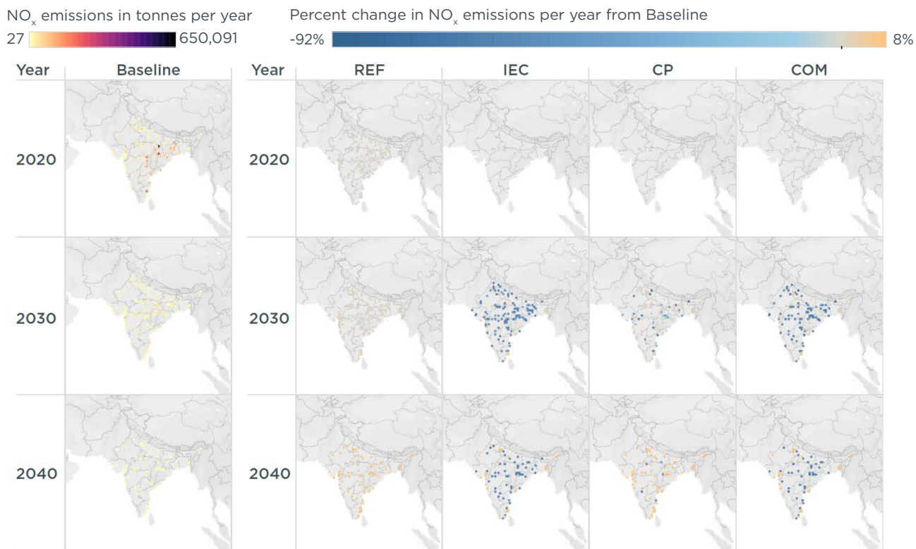
Figure 11. Gridded NO x emissions from power plants. Results for the REF, IEC, CP, and COM scenarios are shown as percent changes in emissions from the Baseline scenario for the same year.
